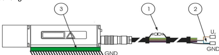
Figure 8 : Isolated Mounting
