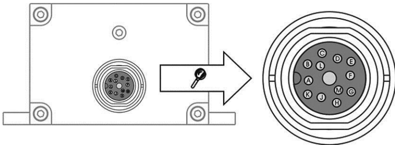
Figure 5 : View of CLDM41A and CLDM42A pole assignments
