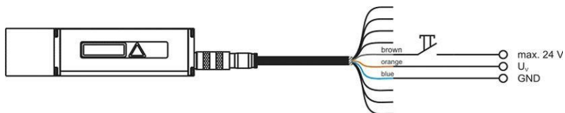
Figure 22 : Wiring diagram of trigger input
