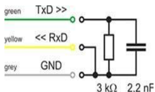
Figure 9 : Recommended terminations wiring for work with open RS-232 left)
