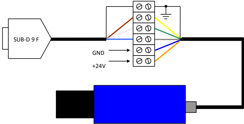
Figure 23 : RS232 cable with power supply for CLDM41A and CLDM42A
